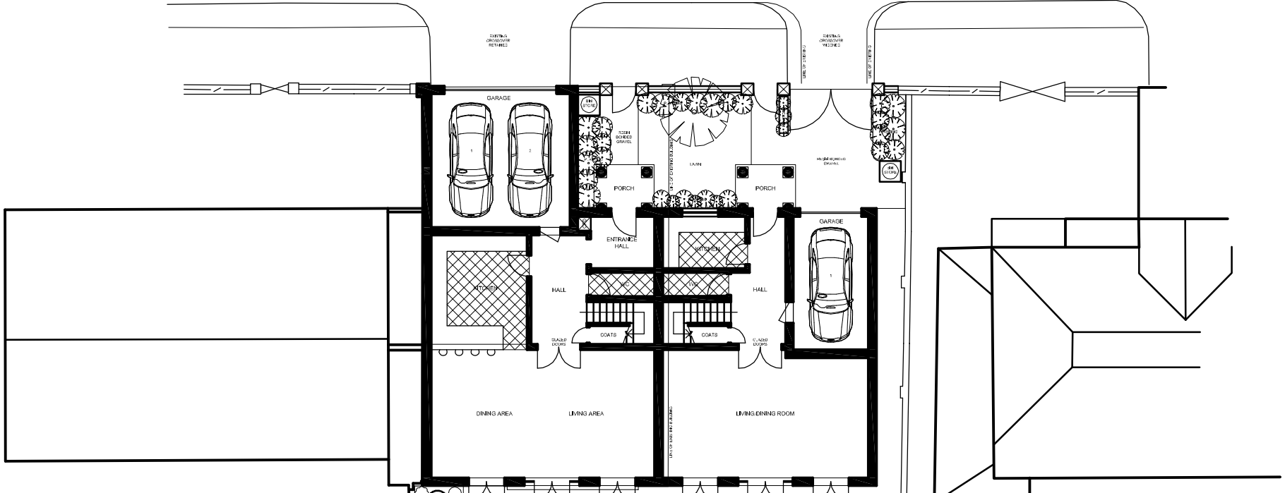
50 Townshend Road PROPOSED GROUND FLOOR PLAN GROSS INTERNAL AREA 106.0m 2
